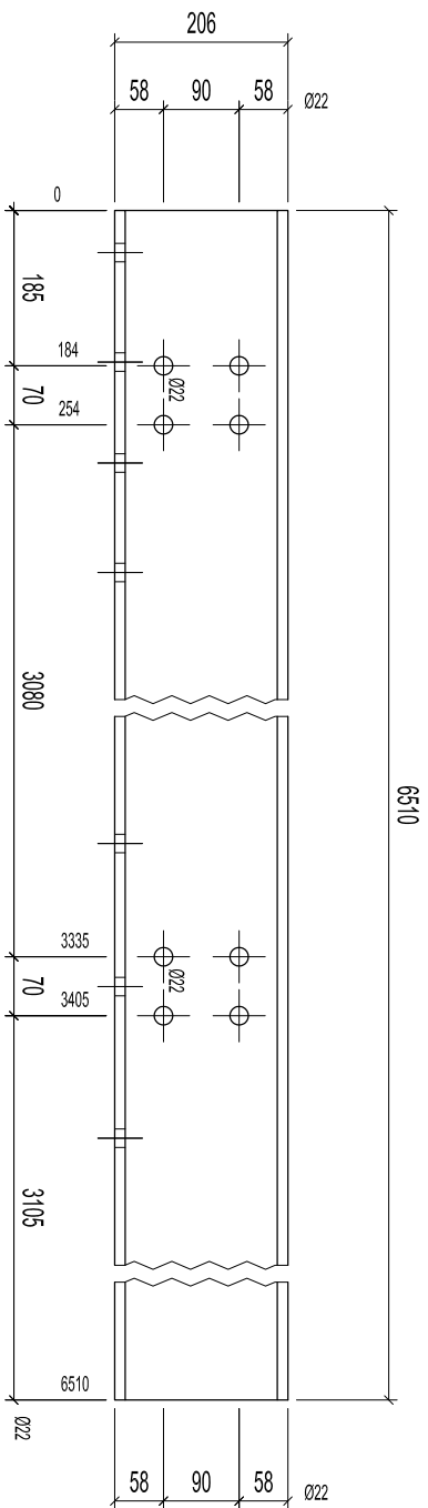
PART - 1005 Front View 200UC52 (2 REQ'D)
