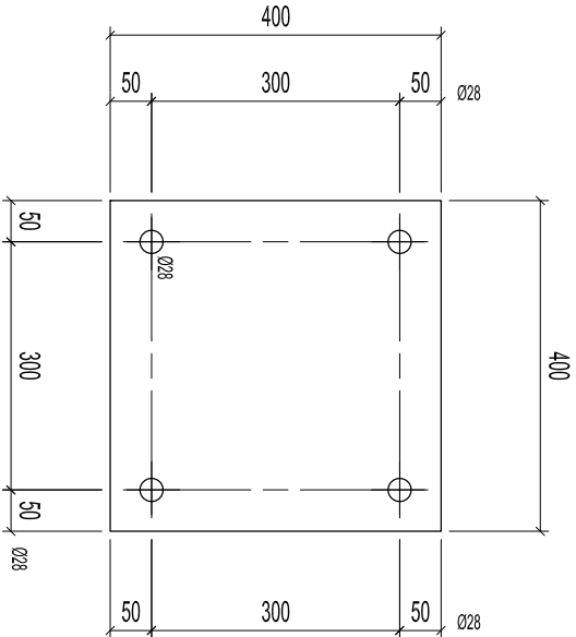
PART - 1138 PLATE 400X25 (11 REQD)
