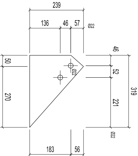
PART - 1139 PLATE 239X10 (4 REQ'D)
